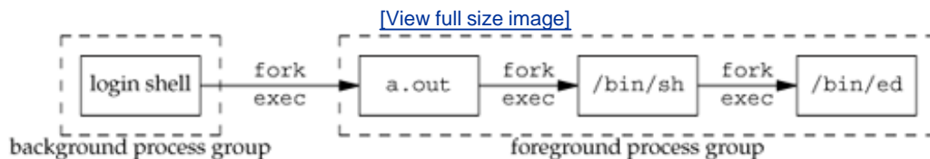
Figure 10.27. Foreground and background process groups for Figure 10.26
