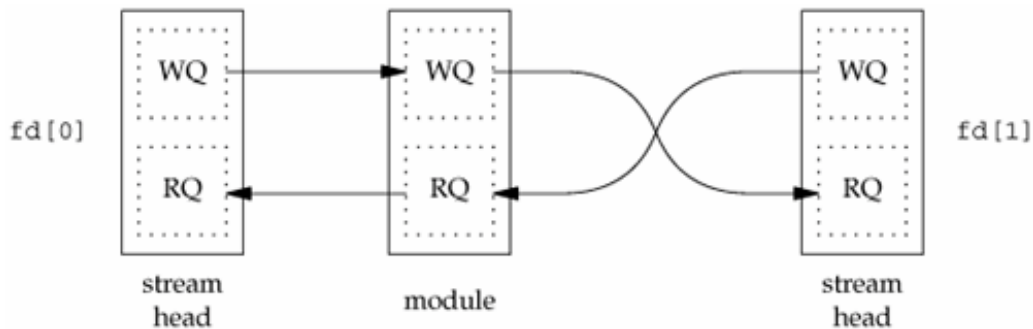
Figure 17.3. Inside a STREAMS pipe with a module
