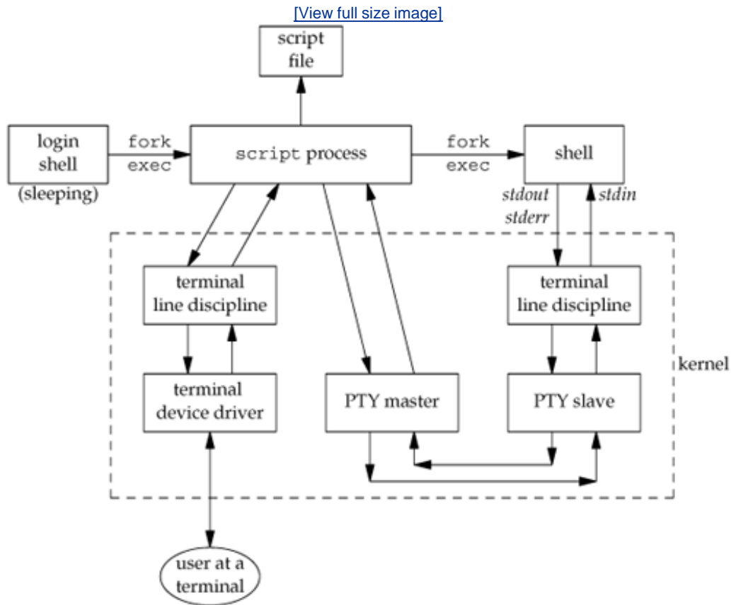
Figure 19.4. The script program
