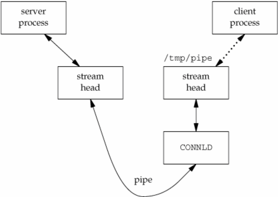
Figure 17.8. Setting up connld for unique connections
