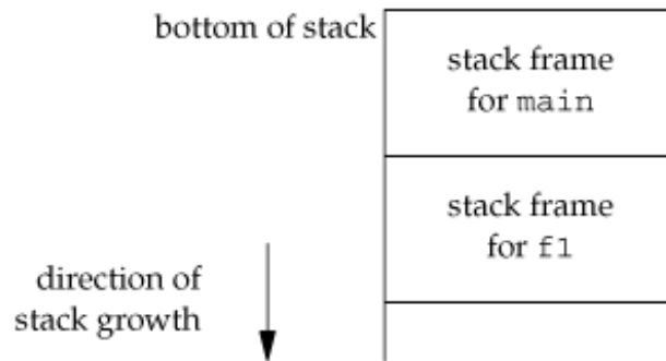
Figure C.8. Stack frames when vfork is called
