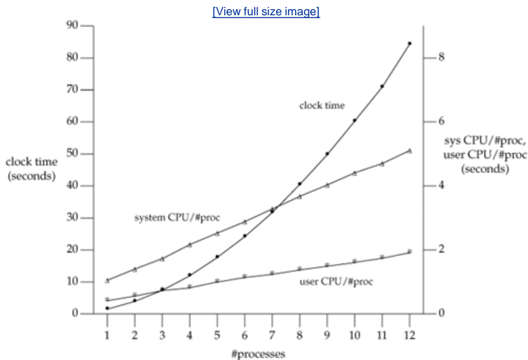
Figure 20.9. Values from Figure 20.8 for advisory fine-grained locking
