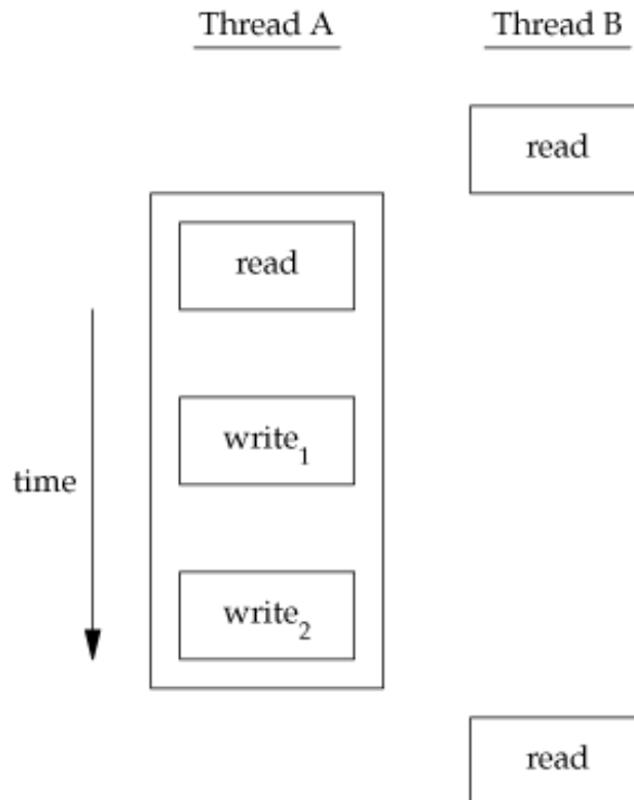
Figure 11.8. Two threads synchronizing memory access
