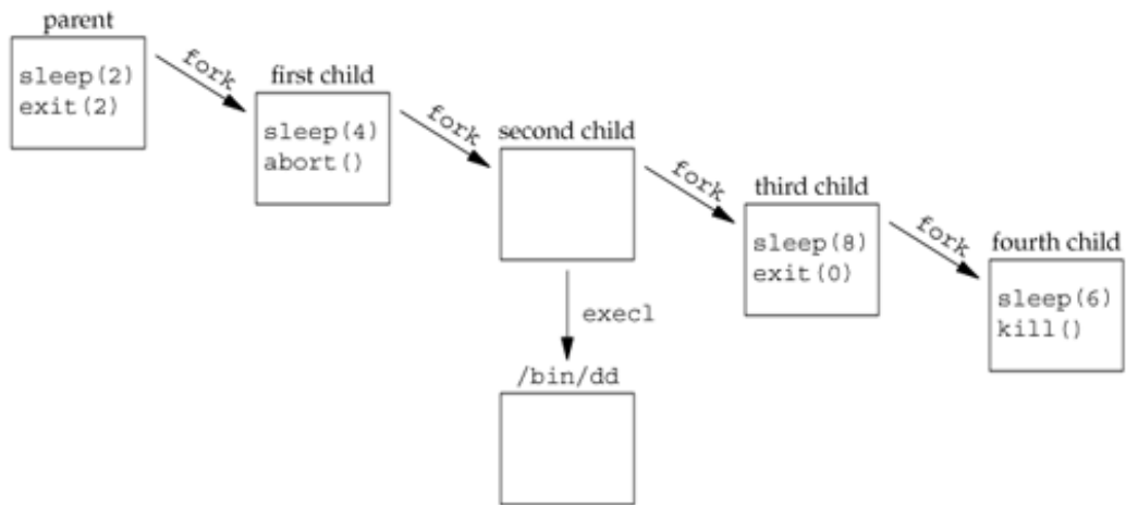
Figure 8.28. Program to generate accounting data
