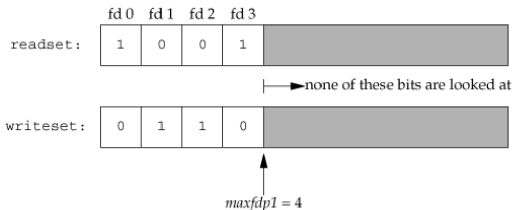
Figure 14.24. Example descriptor sets for select
