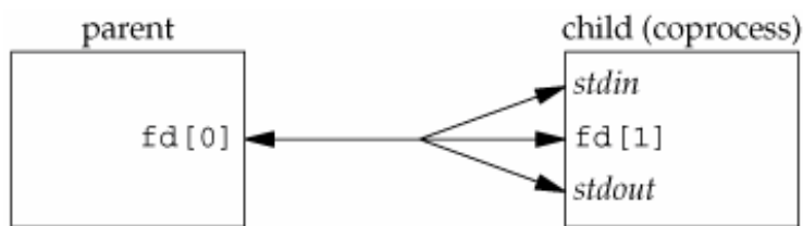
Figure 17.5. Arrangement of descriptors for coprocess
