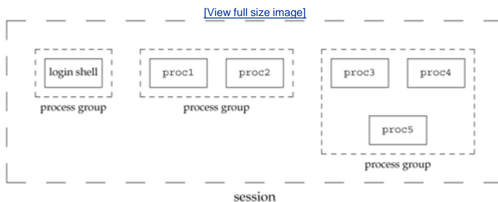
Figure 9.6. Arrangement of processes into process groups and sessions
