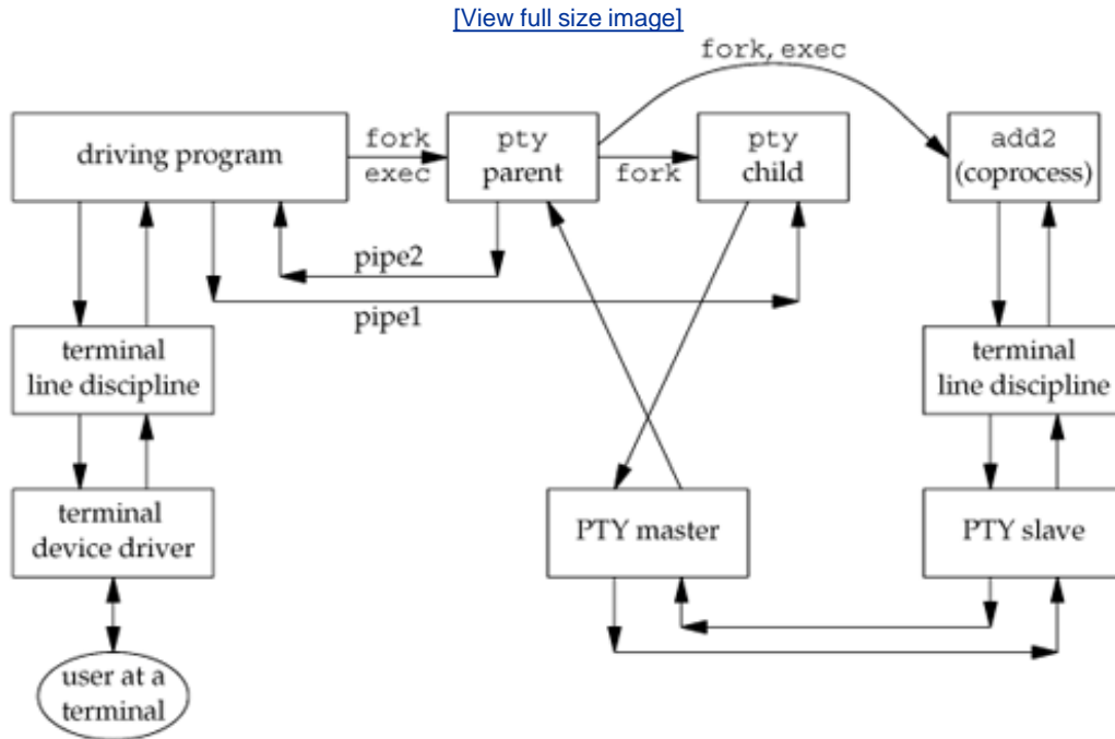
Figure 19.16. Running a coprocess with a pseudo terminal as its input and output
