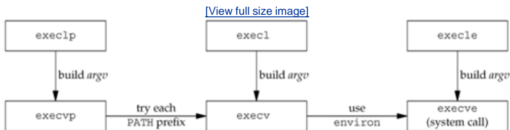
Figure 8.15. Relationship of the six exec functions
