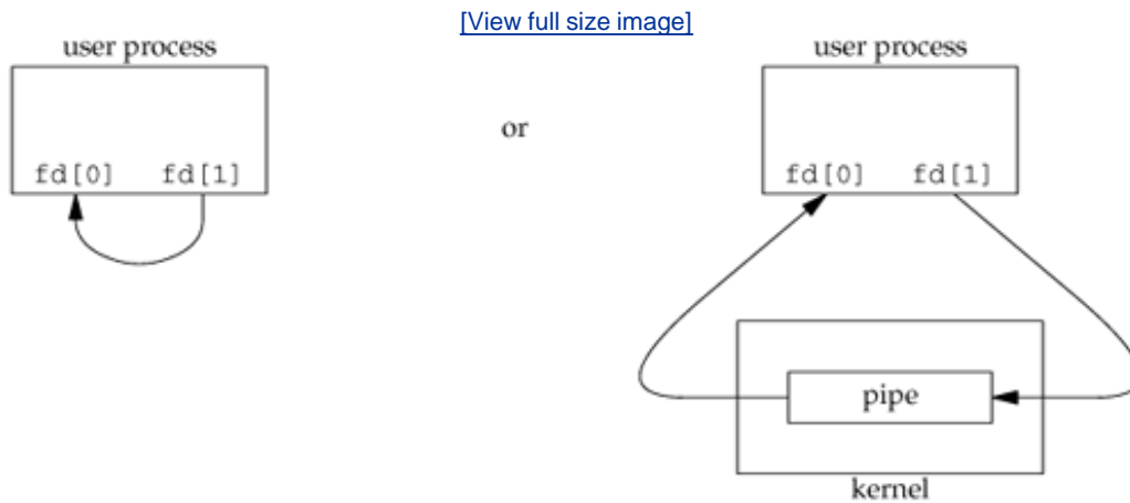
Figure 15.2. Two ways to view a half-duplex pipe
