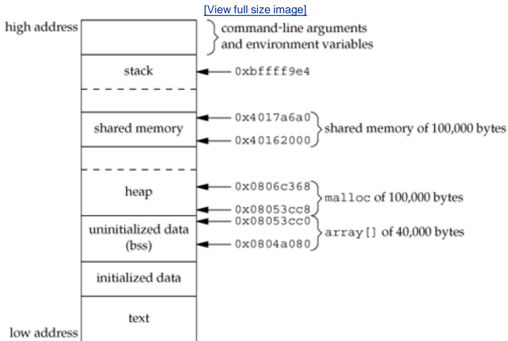
Figure 15.32. Memory layout on an Intel-based Linux system
