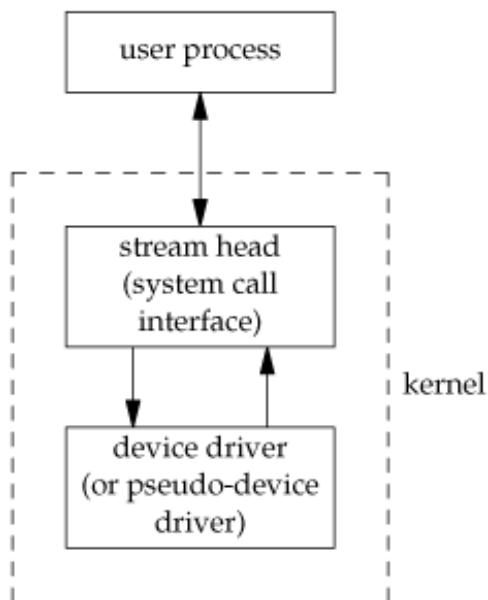
Figure 14.13. A simple stream
