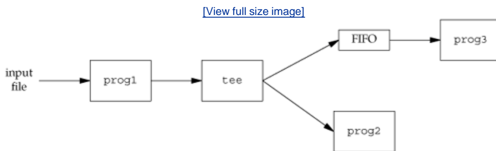
Figure 15.21. Using a FIFO and tee to send a stream to two different processes
