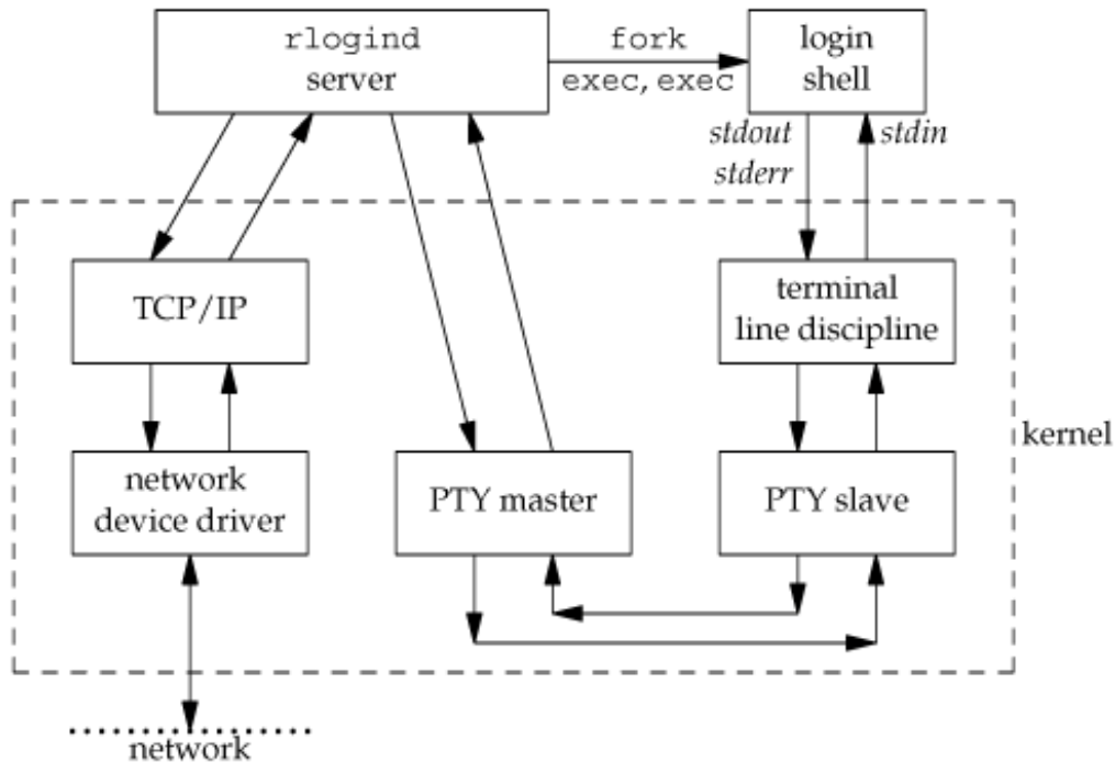
Figure 19.3. Arrangement of processes for rlogind server
