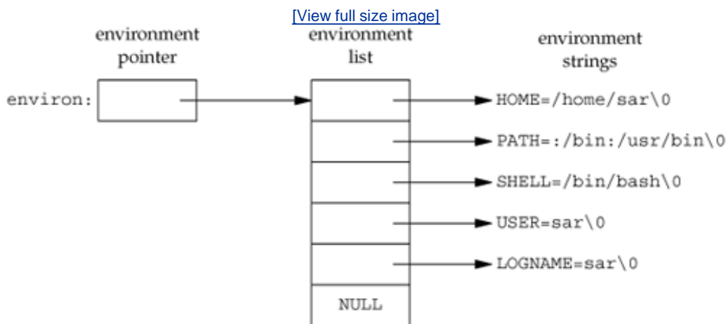
Figure 7.5. Environment consisting of five C character strings
