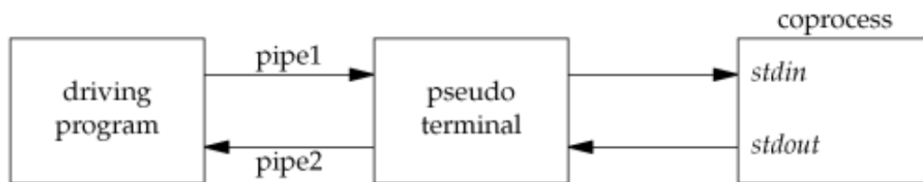
Figure 19.5. Driving a coprocess using a pseudo terminal
