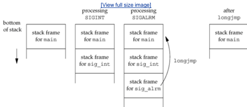
Figure C.10. Stack frames before and after longjmp
