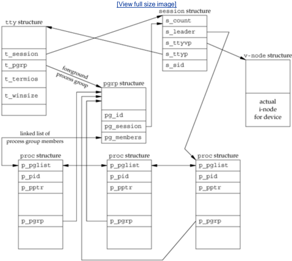
Figure 9.12. FreeBSD implementation of sessions and process groups
