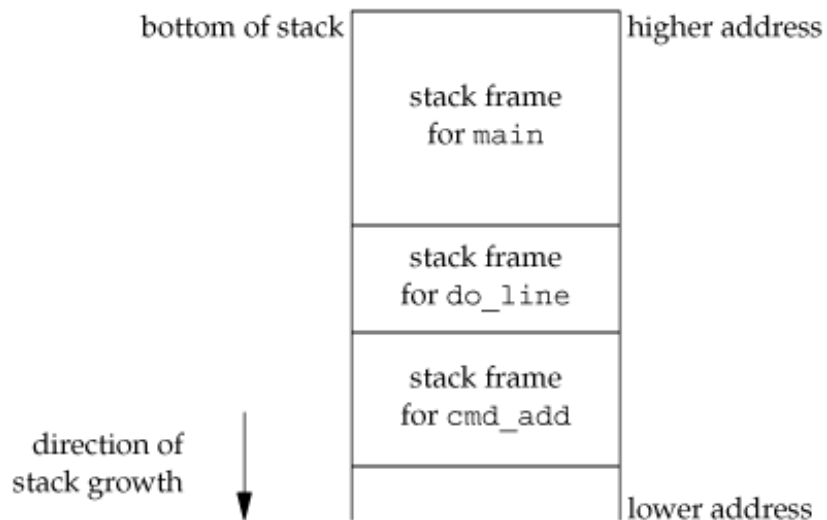
Figure 7.10. Stack frames after cmd_add has been called
