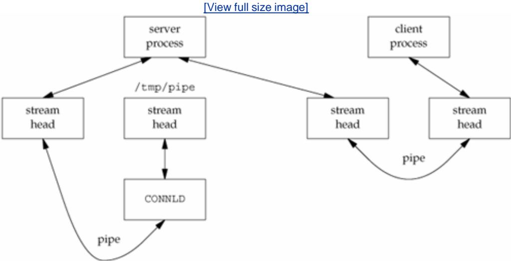
Figure 17.9. Using connld to make unique connections
