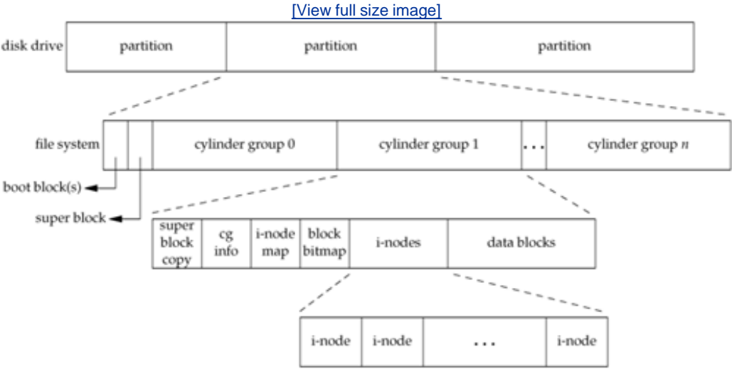
Figure 4.13. Disk drive, partitions, and a file system
