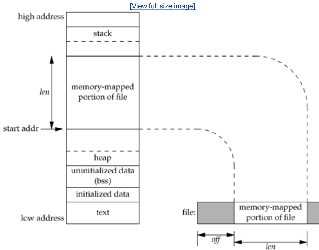
Figure 14.31. Example of a memory-mapped file
