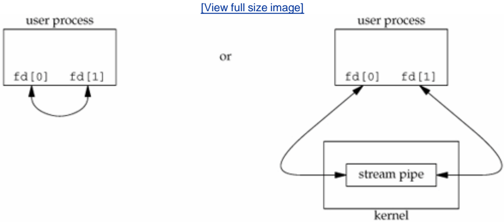
Figure 17.1. Two ways to view a STREAMS pipe
