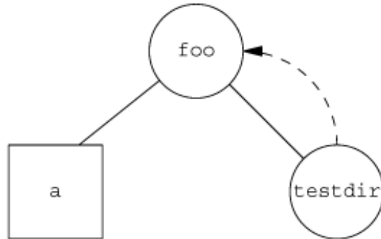
Figure 4.18. Symbolic link testdir that creates a loop
