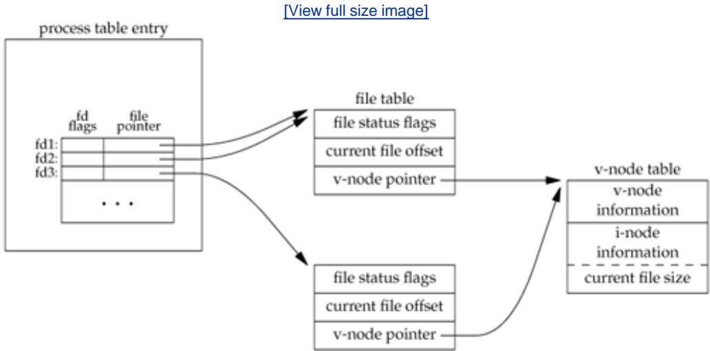
Figure C.2. Result of dup and open
