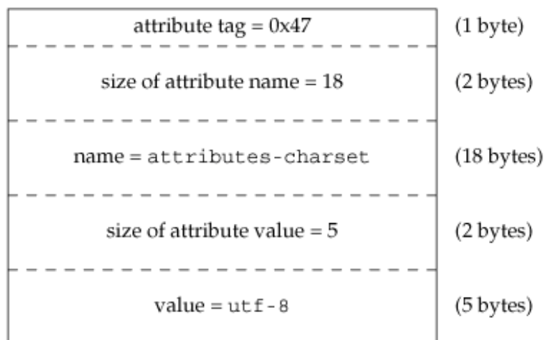
Figure 21.3. Sample IPP attribute encoding
