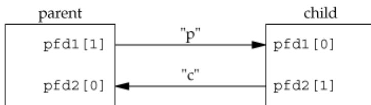
Figure 15.8. Using two pipes for parentchild synchronization
