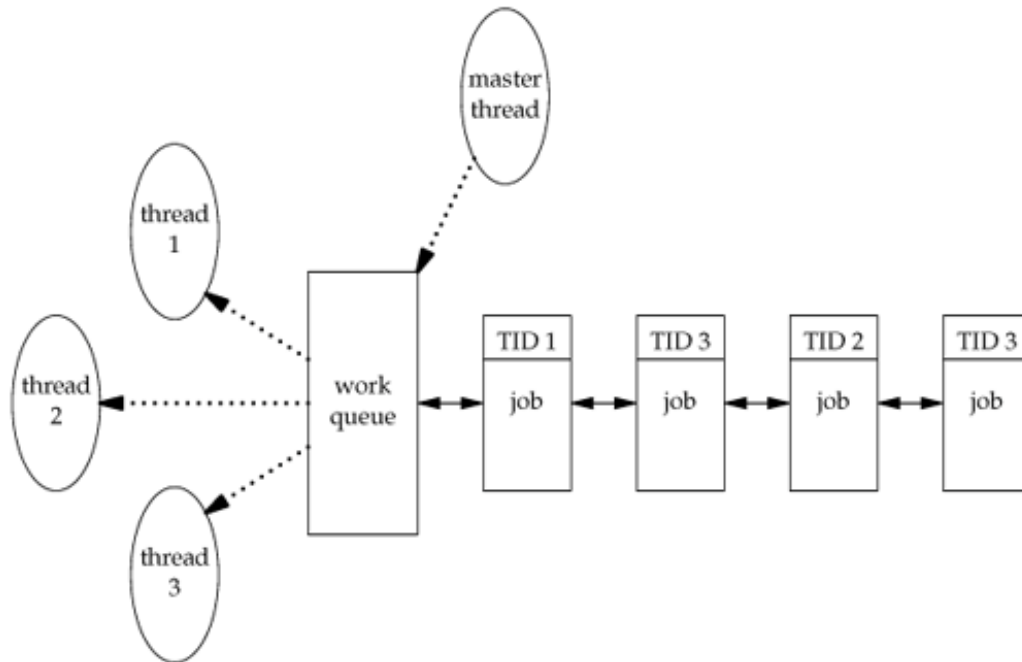
Figure 11.1. Work queue example
