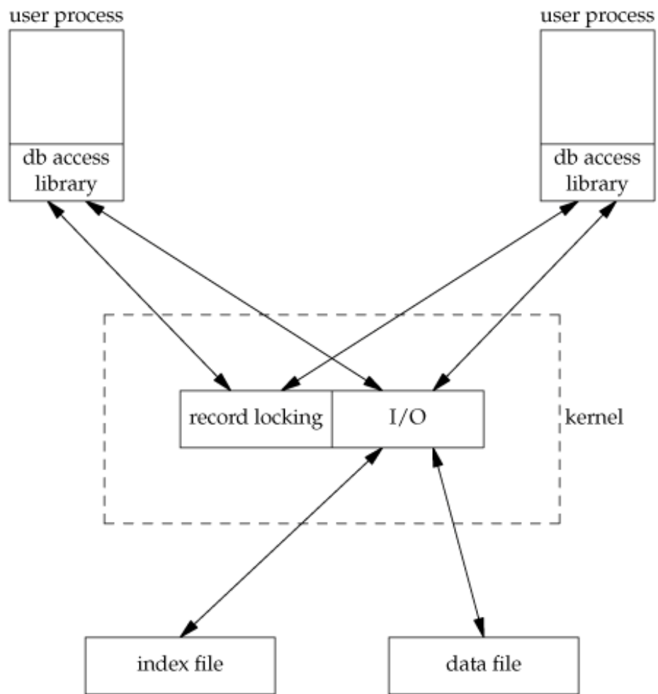
Figure 20.5. Decentralized approach for database access
