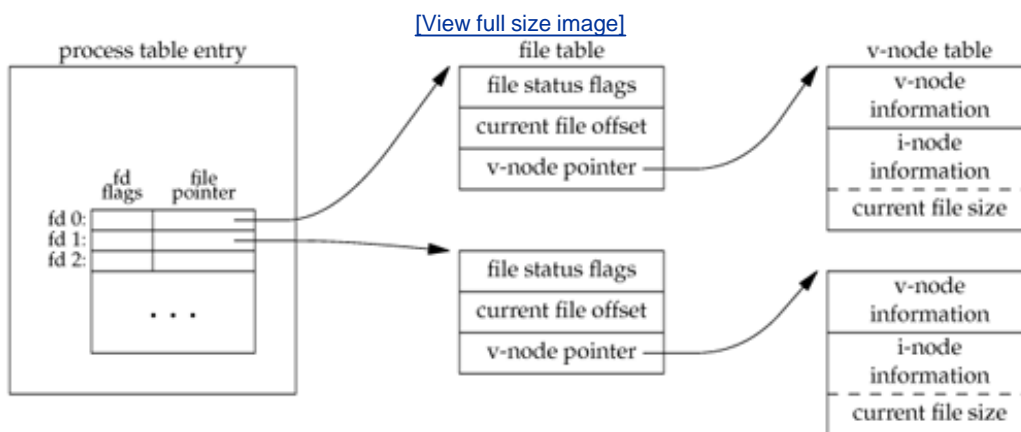
Figure 3.6. Kernel data structures for open files
