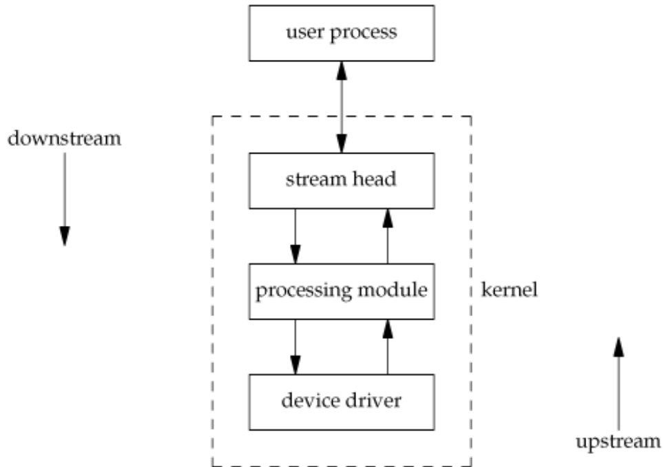
Figure 14.14. A stream with a processing module
