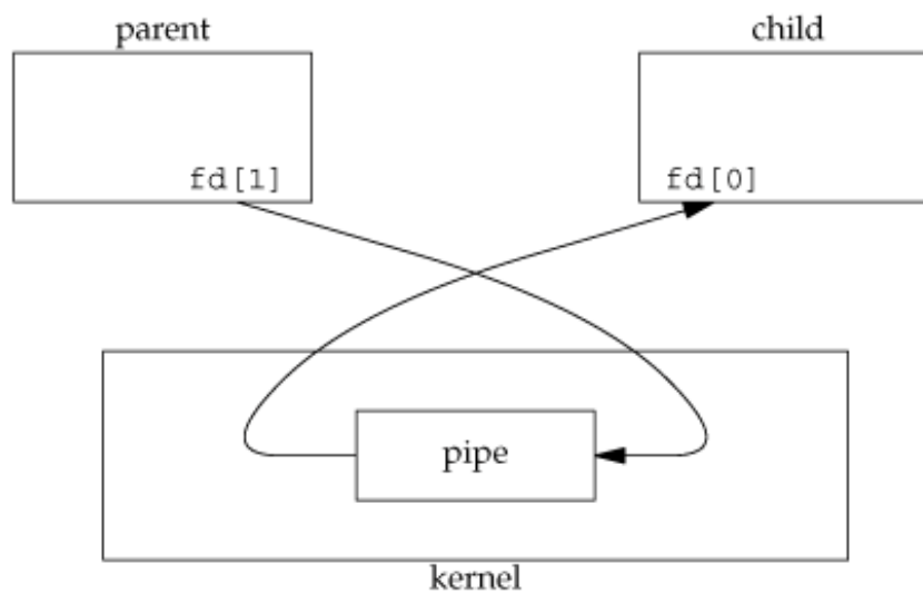
Figure 15.4. Pipe from parent to child
