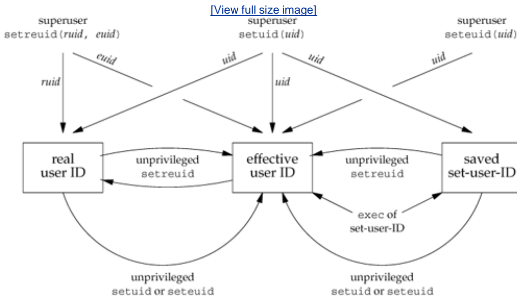
Figure 8.19. Summary of all the functions that set the various user IDs
