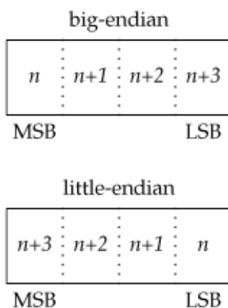
Figure 16.4. Byte order in a 32-bit integer
