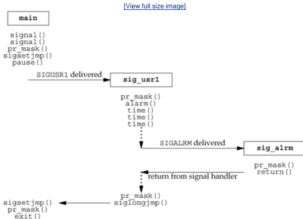
Figure 10.21. Time line for example program handling two signals
