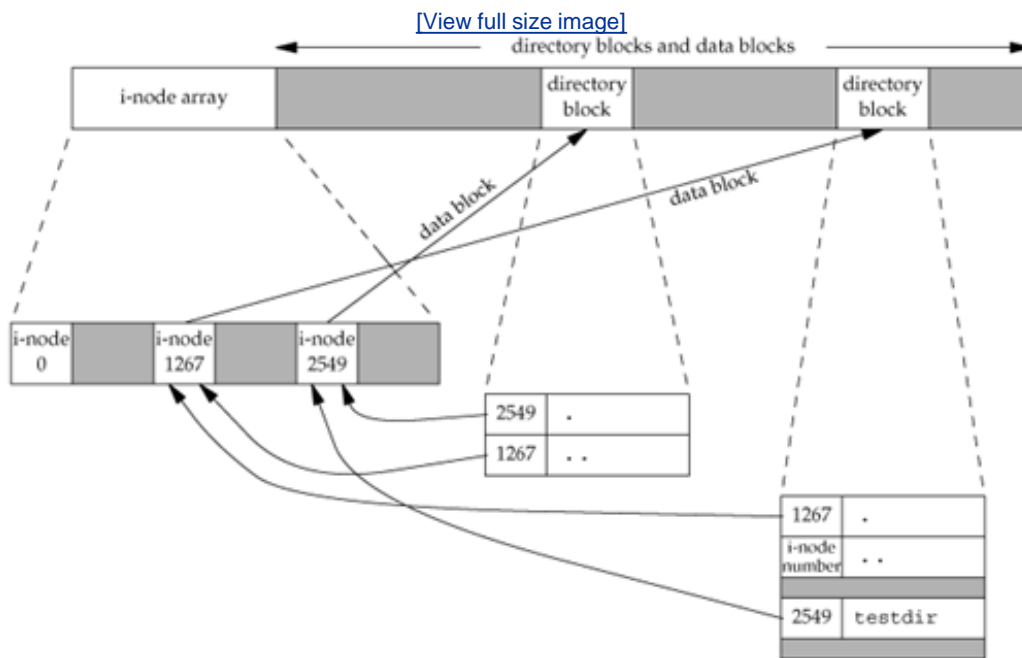
Figure 4.15. Sample cylinder group after creating the directory testdir
