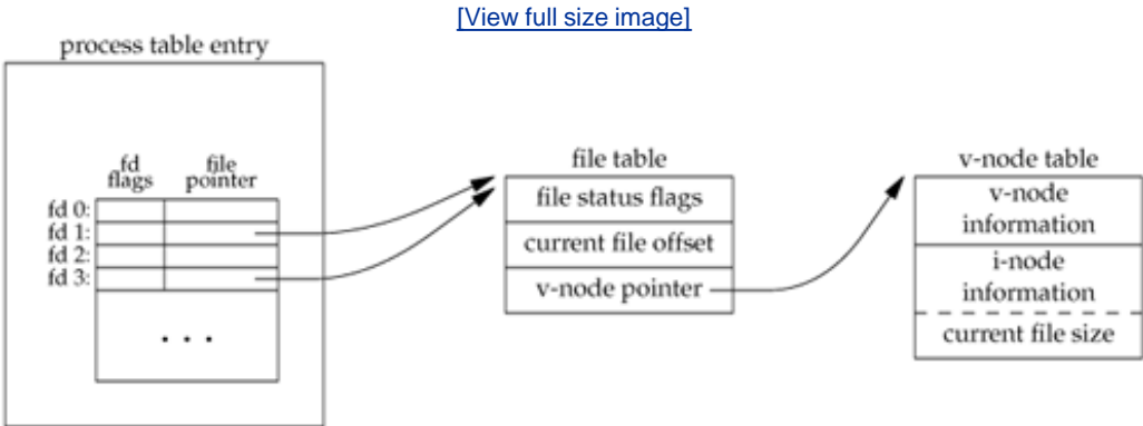
Figure 3.8. Kernel data structures after dup(1)
